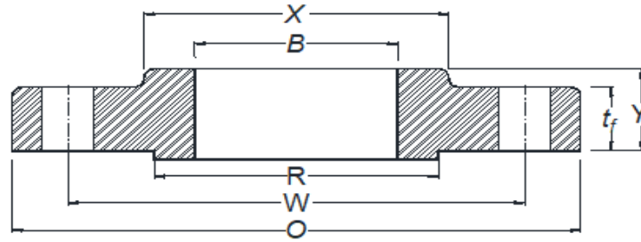
SLIP ON FLANGE
